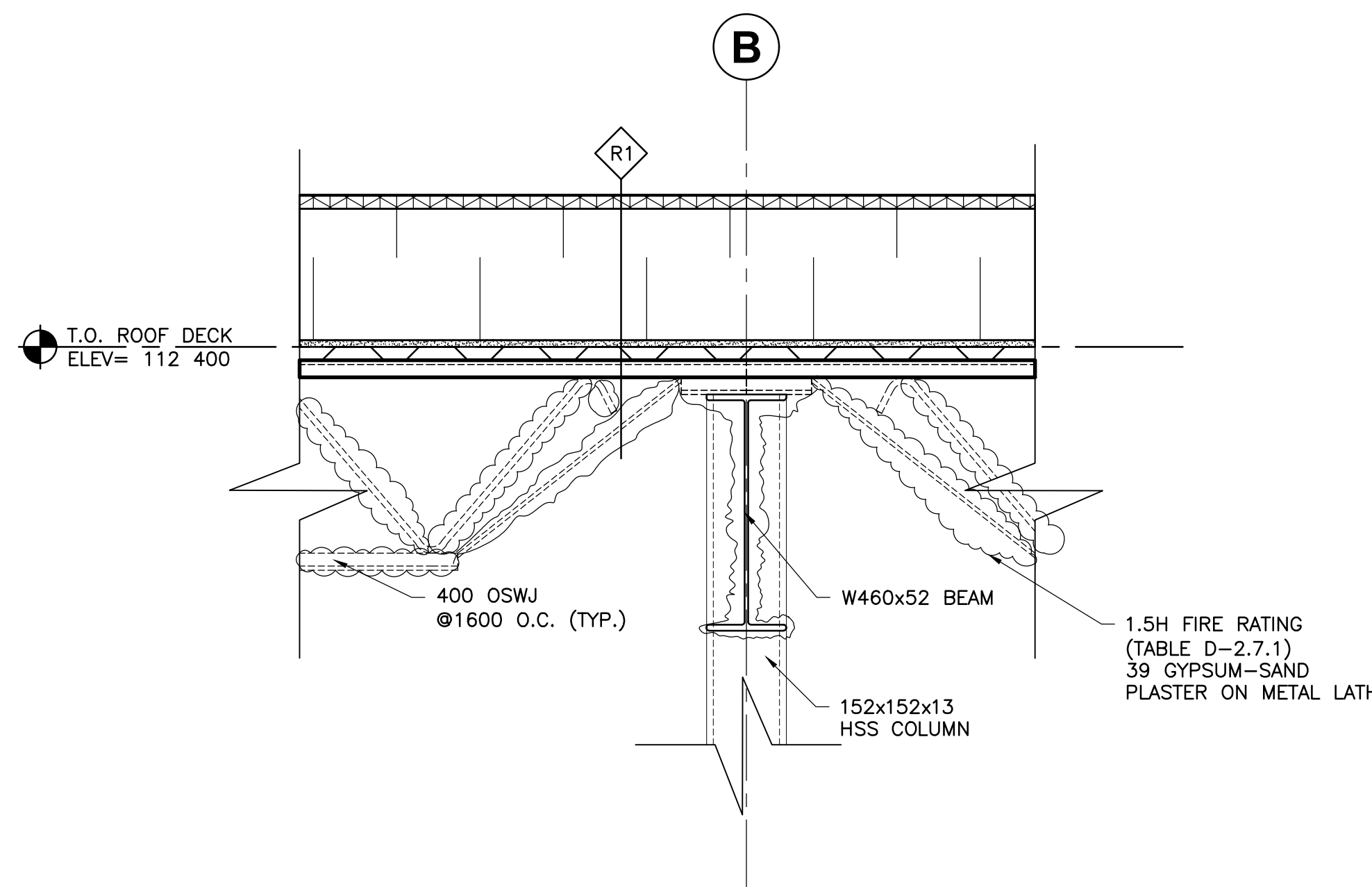
5 SECTION DETAIL @ROOF A7 SCALE = 1:10
