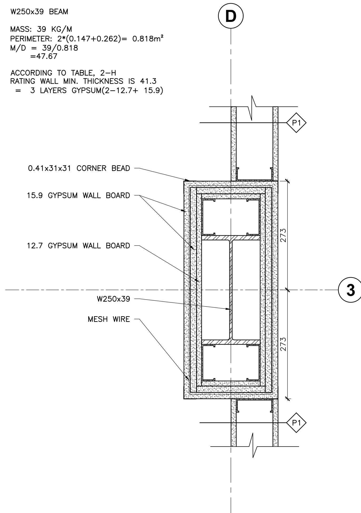
3 2-HR FIRE RATED COLUMN DETAIL A7 SCALE = 1:5
