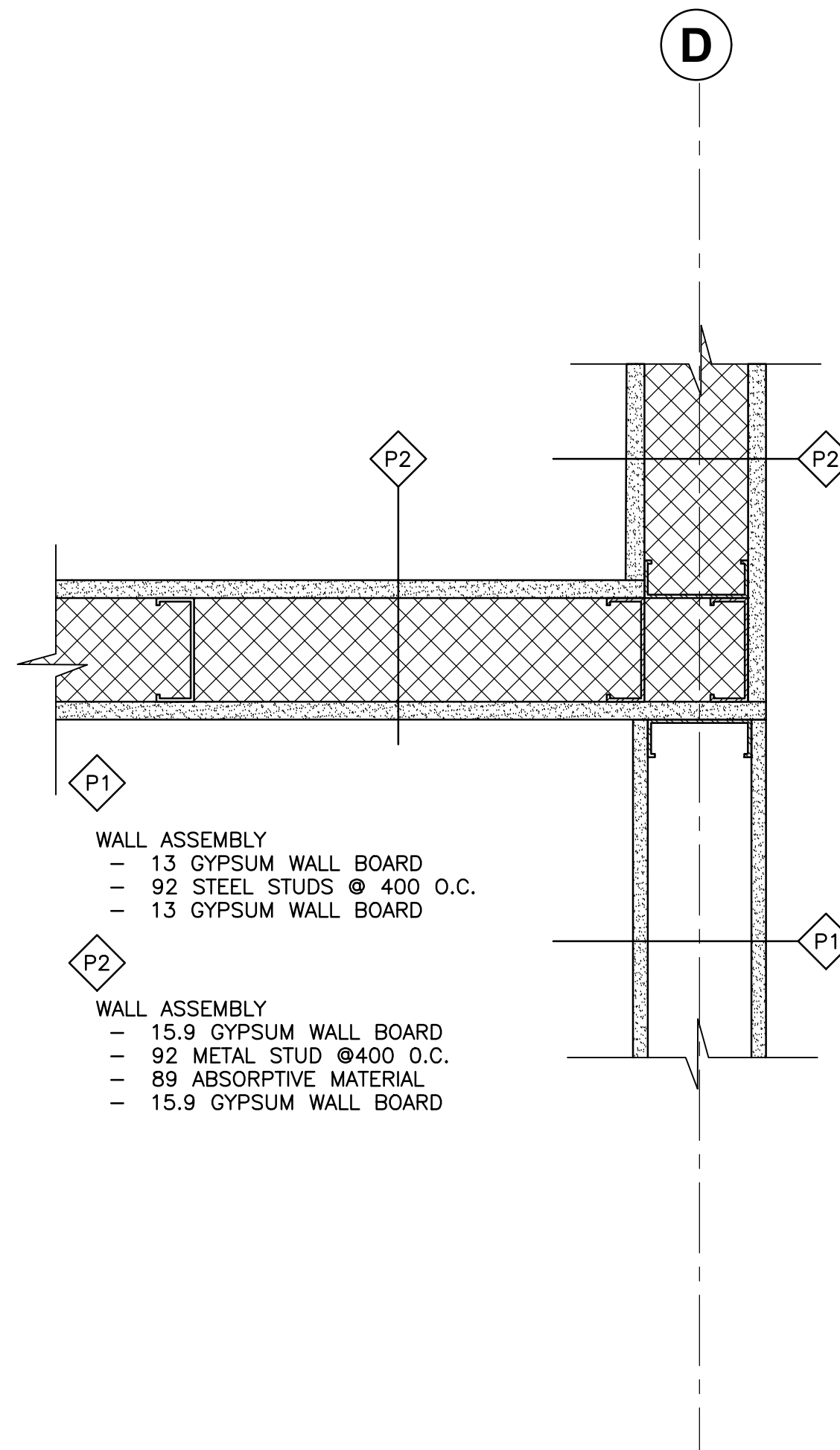
2 PLAN DETAIL 1 A7 SCALE = 1:5
