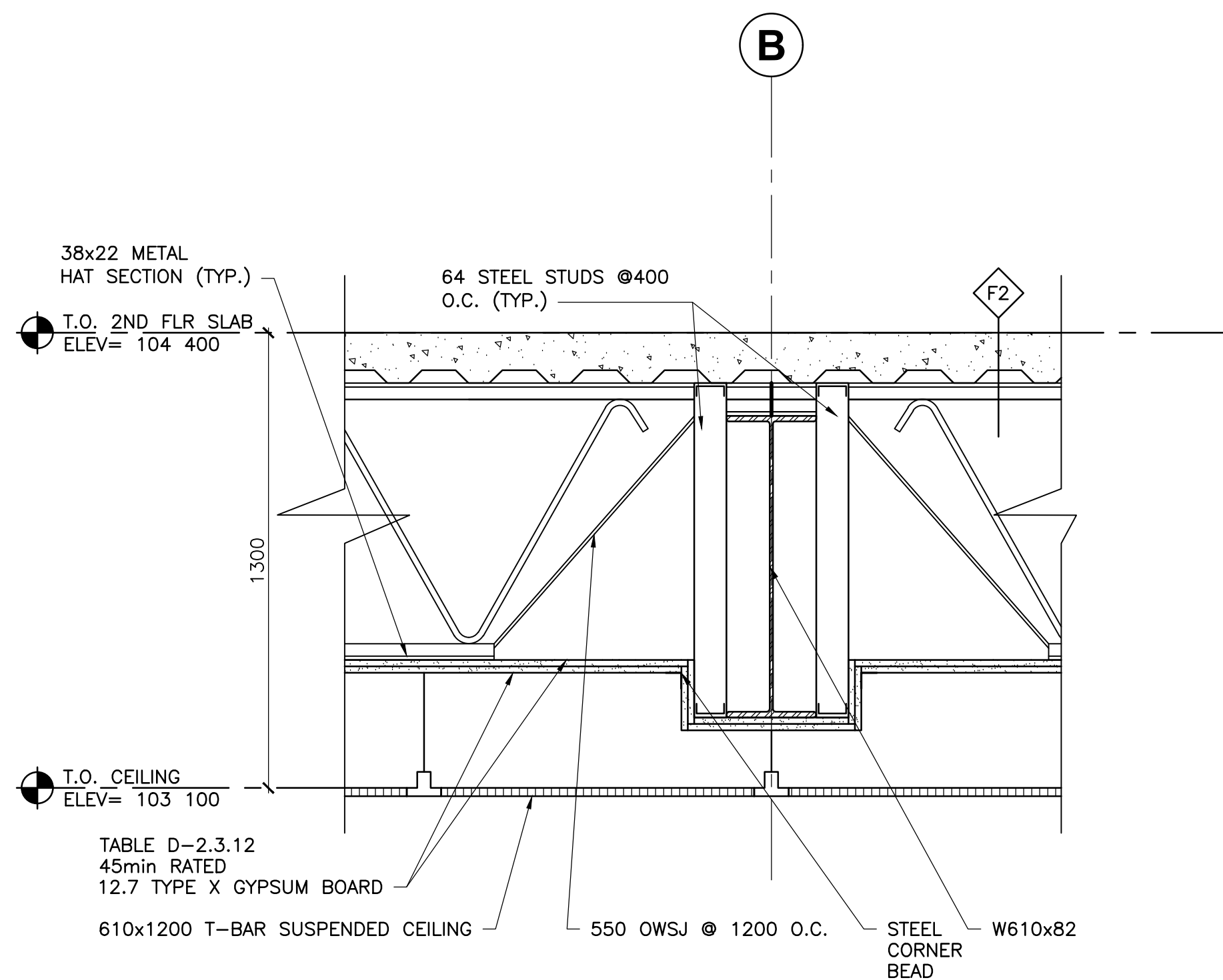
4 SECTION DETAIL @2ND FLOOR A7 SCALE = 1:10
